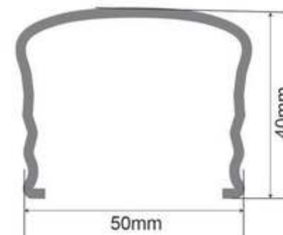
U型葡萄柱 U type vineyard post
